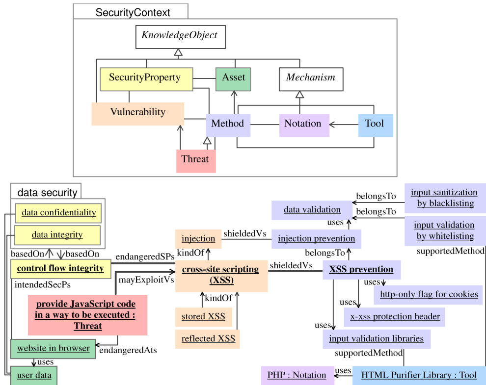
Figure 3. Upper part: SecEval’s Security Context model, serving as a legend for the lower part: SecWAO example of relations regarding cross-site-scripting (XSS).
