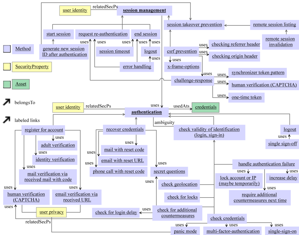
Figure 8. SecWAO methods: Authentication and session management
