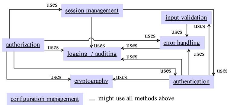
Figure 6. SecWAO: Main methods
