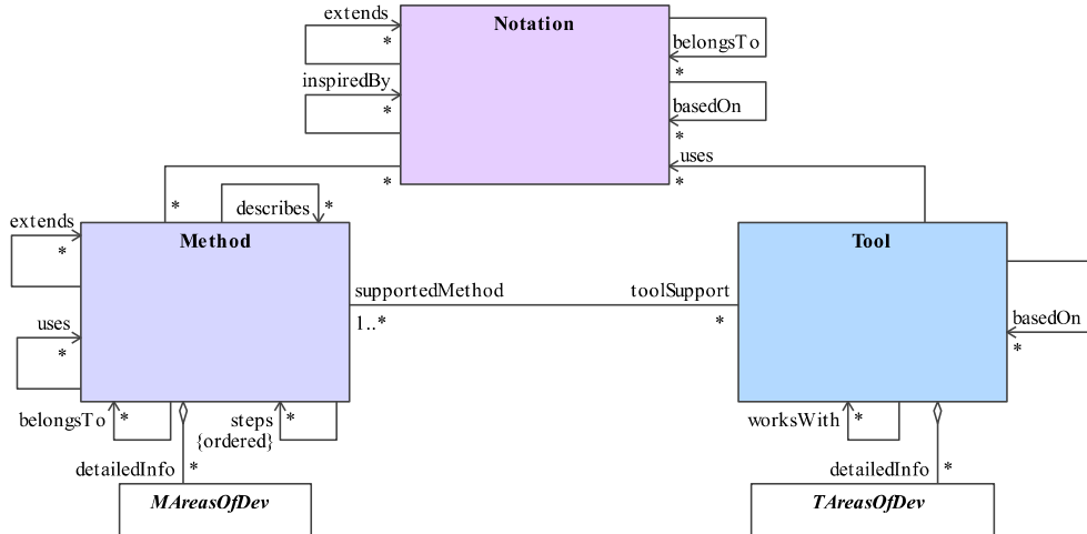
Figure 2. Security Context: Further Associations
