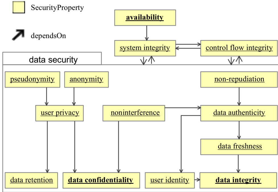
Figure 4. SecWAO Security Properties: Overview
