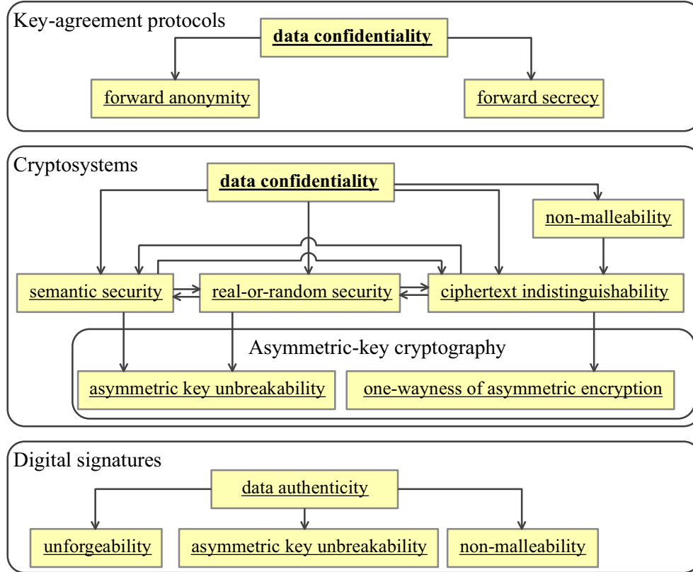
Figure 5. SecWAO Security Properties: Details
