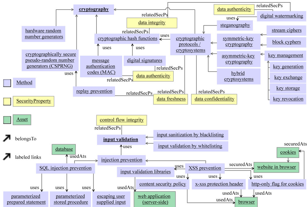
Figure 7. SecWAO methods: Cryptography and input validation
